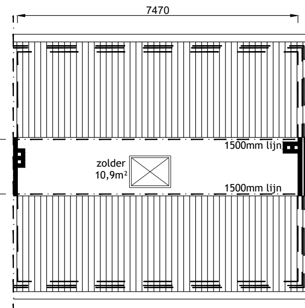
zolder
