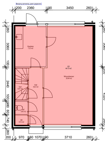
Begane_grond
