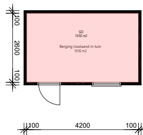
Berging
