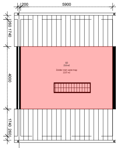
Zolder
