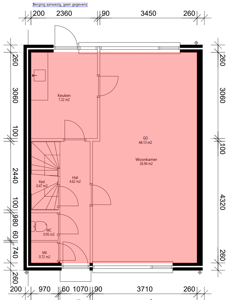
Begane_grond
