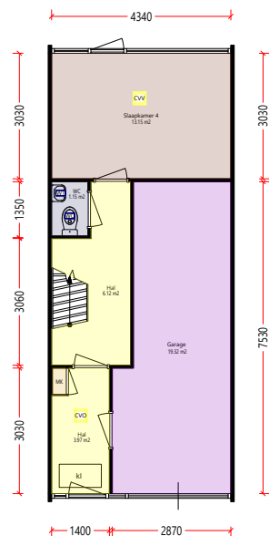
Begane_grond
