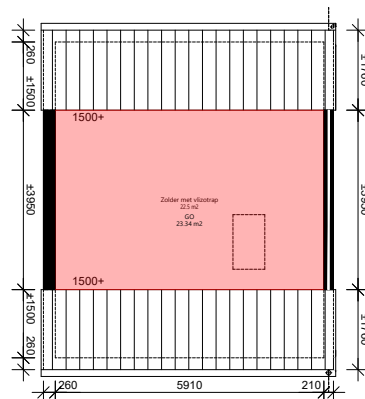
Zolder
