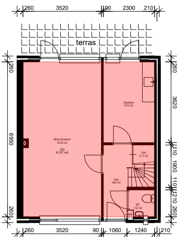
Begane_grond
