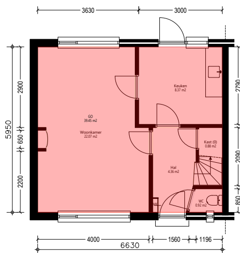
Begane_grond
